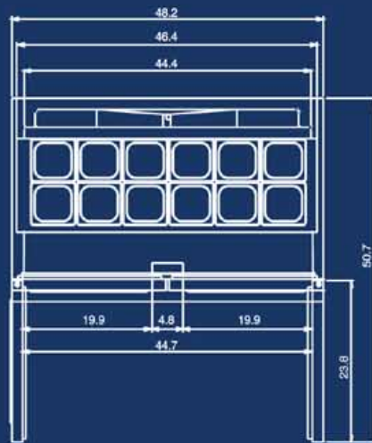
TST-48SD PLAN VIEW
